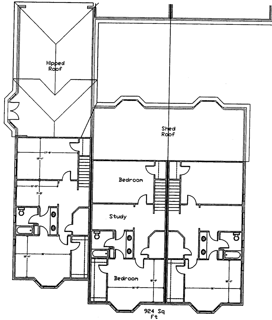
Georgetown Rowhouses Second Floor Plan
