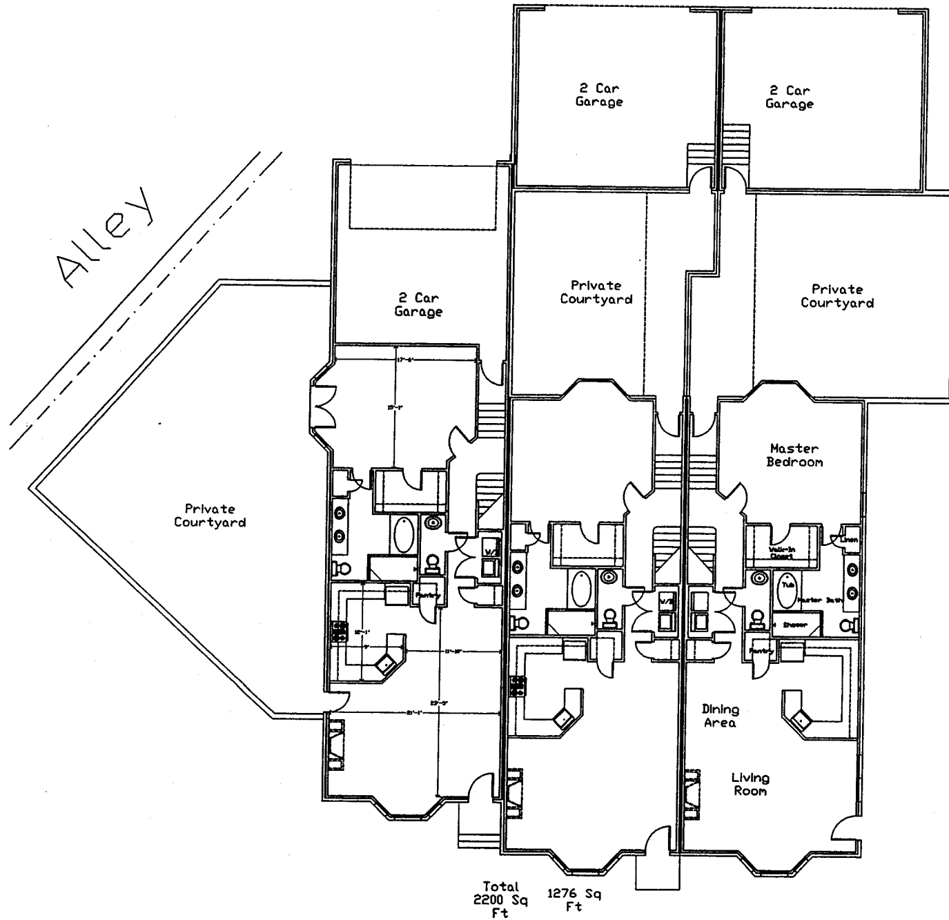
Georgetown Rowhouses First Floor Plan
